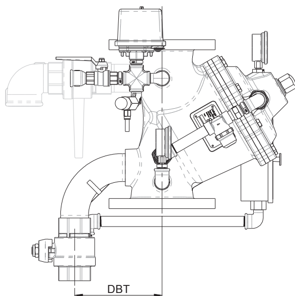
Fig. 5.6.1 - Side view
