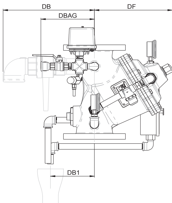
Fig. 5.1.1 - Side view
